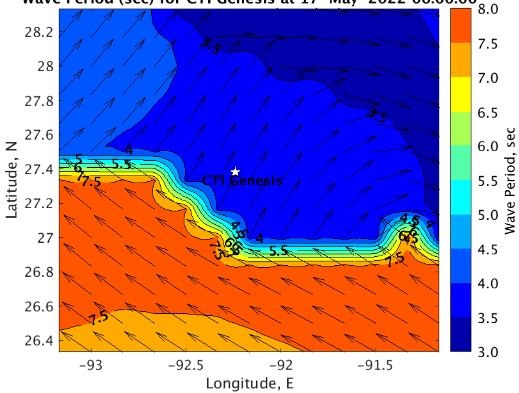
Wave Period (sec) for CTI Genesis at 17-May-2022 06:00:00
